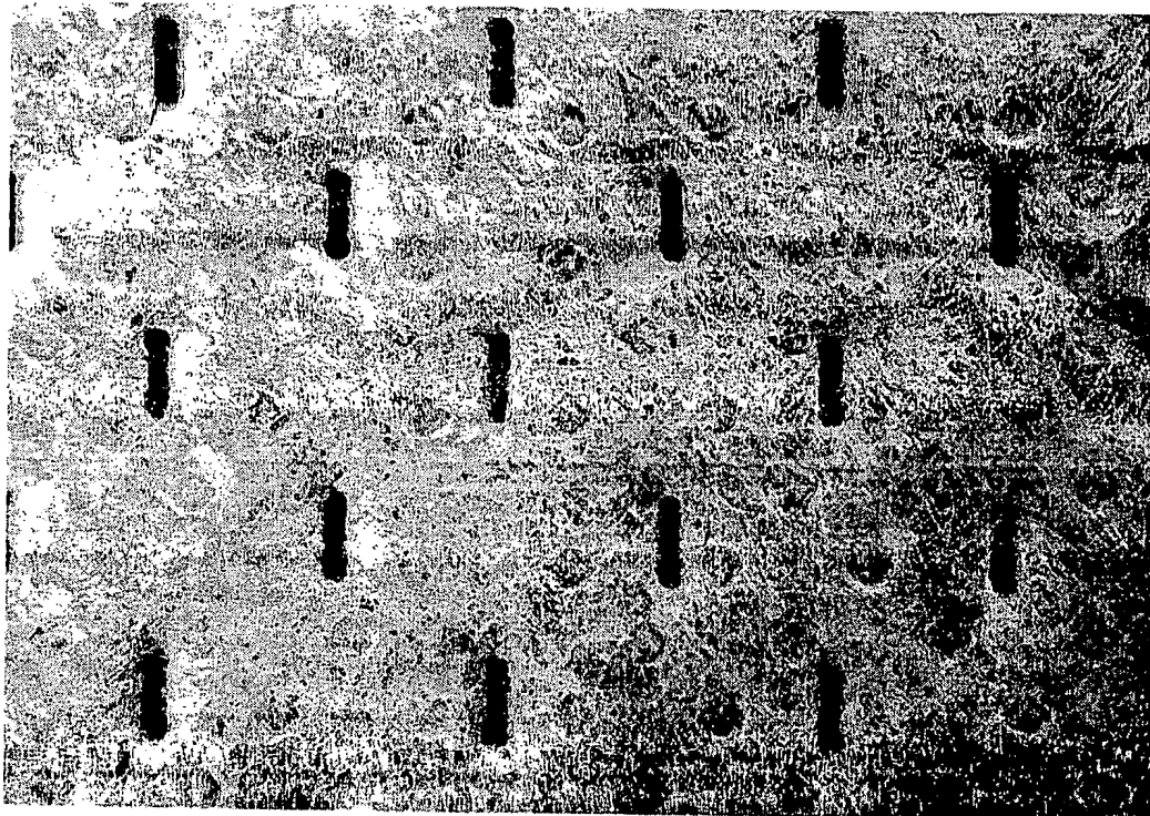
Figure 2. Bond site aspect ratio of 5.
